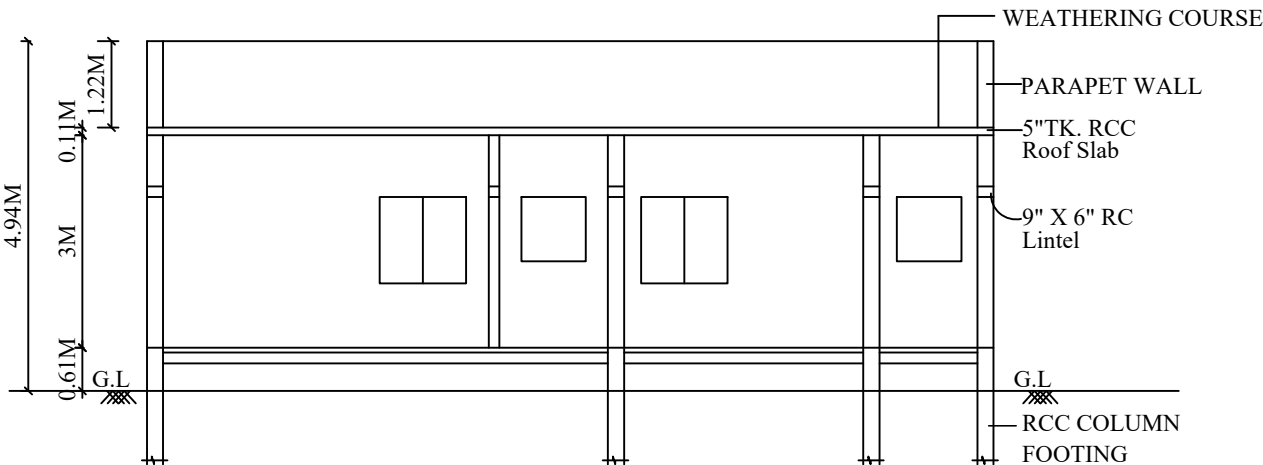
SECTION ON "SP"
