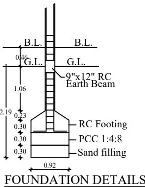
FOUNDATION DETAILS
