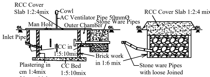
SEPTIC TANK (NTS)
