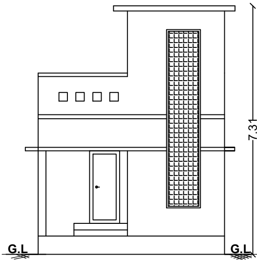
. FRONT ELEVATION .
