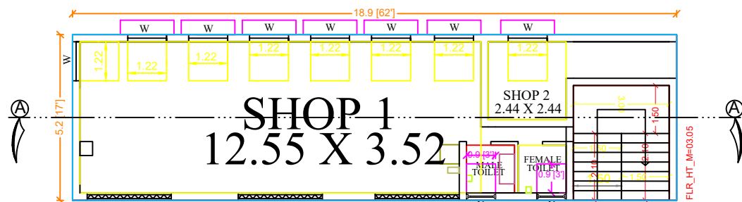
FLOOR PLAN
