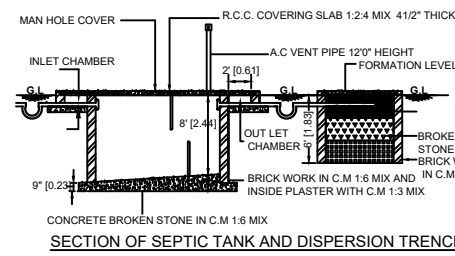
SECTION OF SEPTIC TANK AND DISPERSION TRENCH
