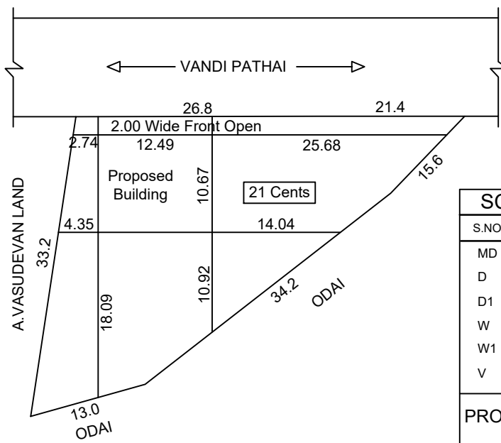
SITE PLAN
