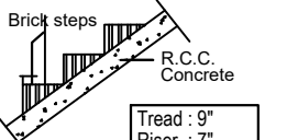
STAIRCASE DETAILS
