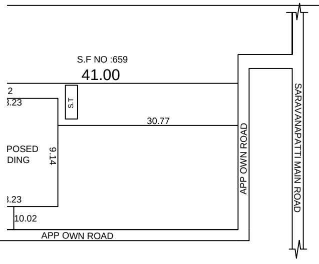
SITE PLAN
