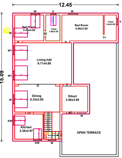
. PROPOSED FIRST FLOOR .
