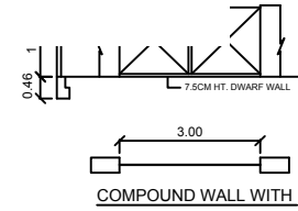
COMPOUND WALL WITH DWARF WALL DETAILS
