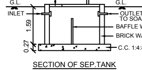
SECTION OF SEPT.TANK
