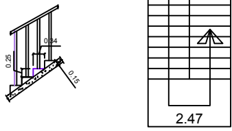
STAIRCASE DETAILS
