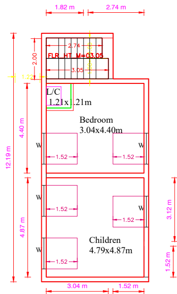
PROP. SECOND FLOOR PLAN
