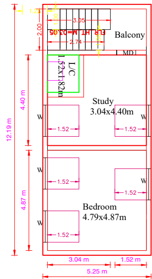
PROP. FIRST FLOOR PLAN
