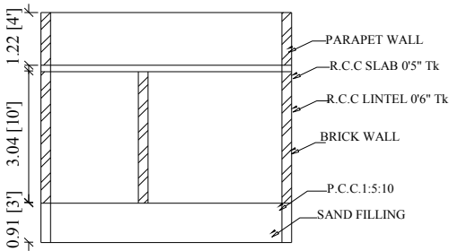
SECTION ON"AB"
