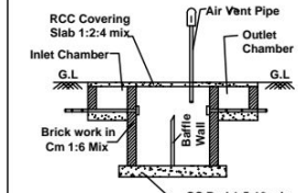
SECTION ON SEPTIC TANK AND DISPERSION TRENCH (NOT TO SCALE)
