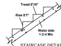
STAIRCASE DETAILS (NOT TO SCALE)
