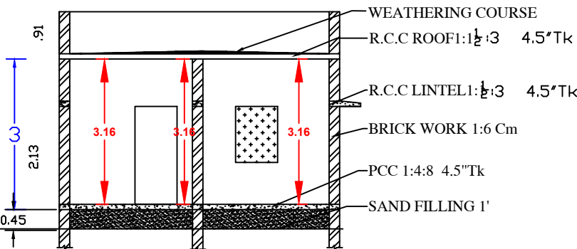
CUT SECTION ON AB
