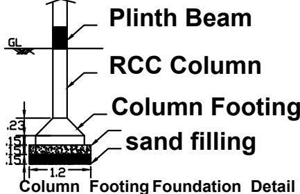
Column Footing Foundation Detail
