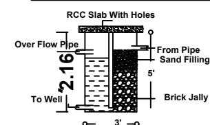
RWHS Tank Details
