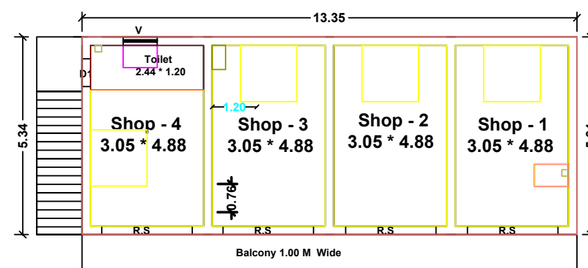
PLAN - GROUND FLOOR
