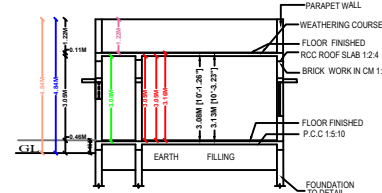
SECTION "A-B"
