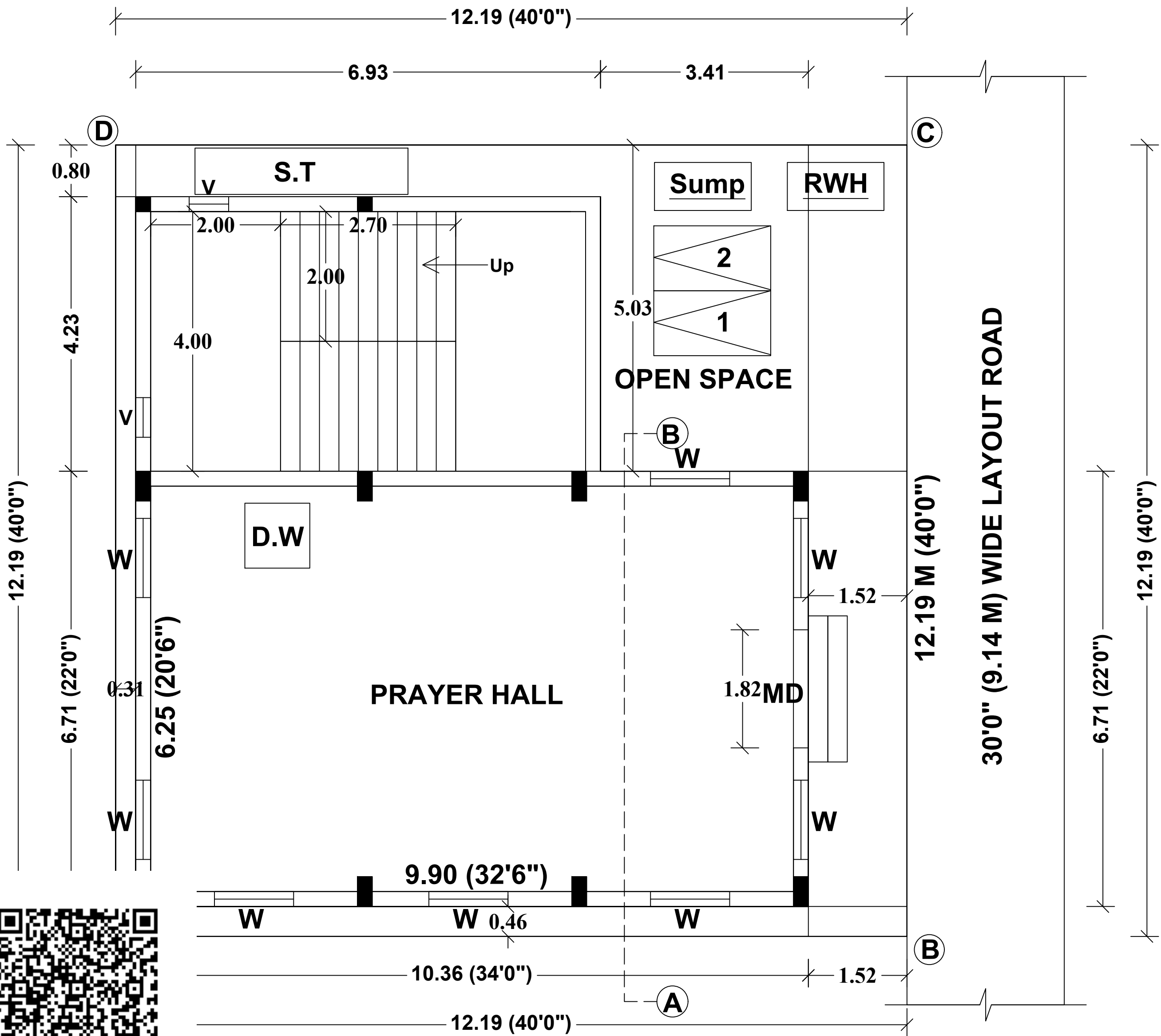
.SITE PLAN & GROUND FLOOR PLAN.
