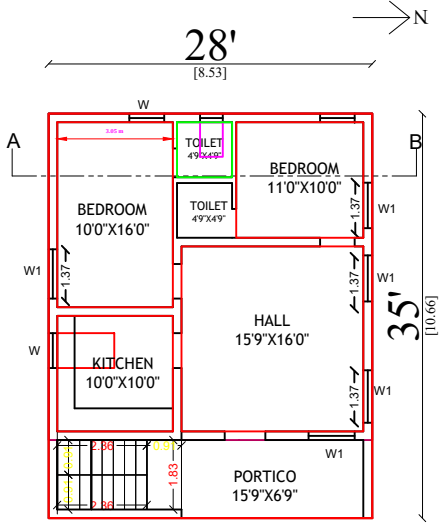
GROUND FLOOR PLAN (EAST FACING) 980.00 SQF
