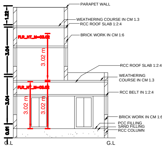
SECTION ON AA & BB
