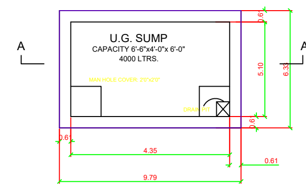
SUMP DETAIL
