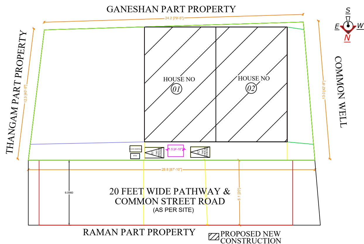
SITE PLAN FOR SURVEY NO. 560/2C1
