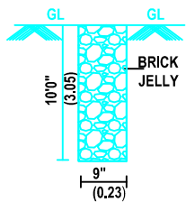
PERCULATION PIT
