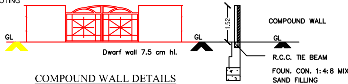
COMPOUND WALL DETAILS
