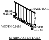
STAIRCASE DETAILS
