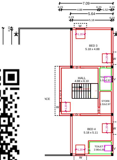
PROPOSED FIRST FLOOR PLAN (NORTH FACING)
