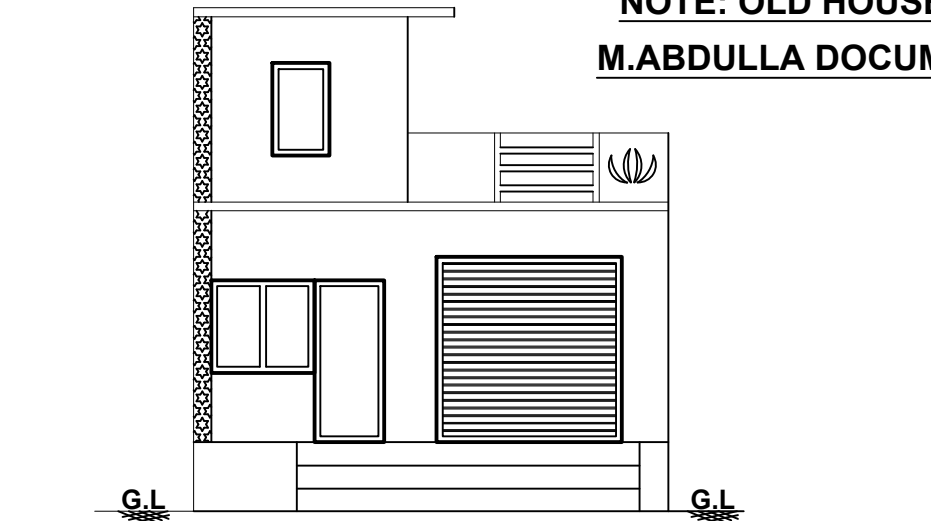
. FRONT ELEVATION .
