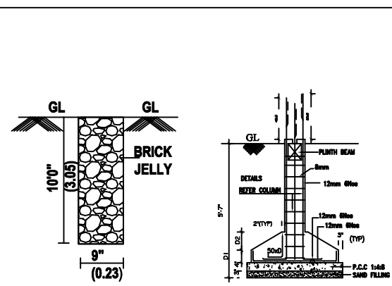
PERCOLATION PIT FOUNDATION DETAILS
