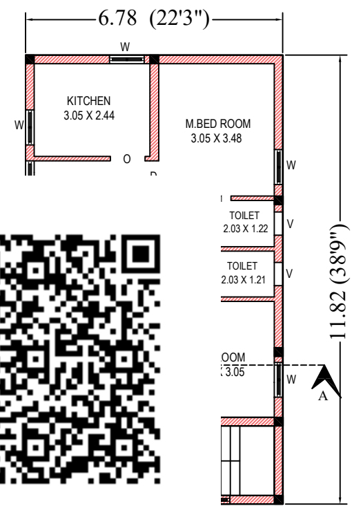
PRO.GROUND FLOOR
