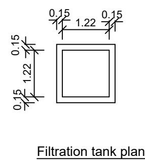
Filtration tank plan
