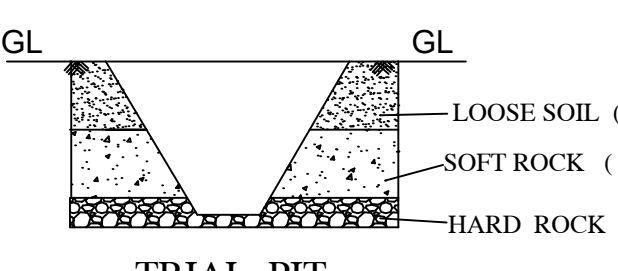
TRIAL PIT
