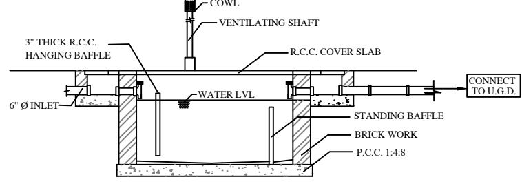
SECTION DETAILS OF SEPTIC TANK
