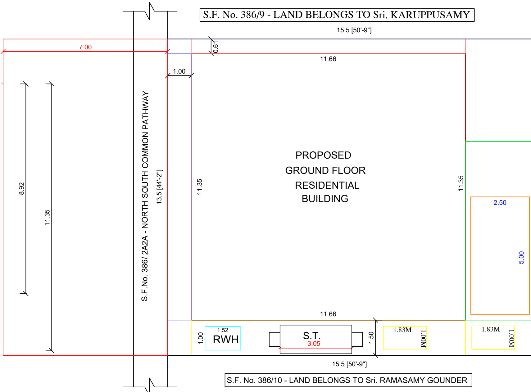
SITE PLAN - MEANT FOR RESIDENTIAL BUILDING
