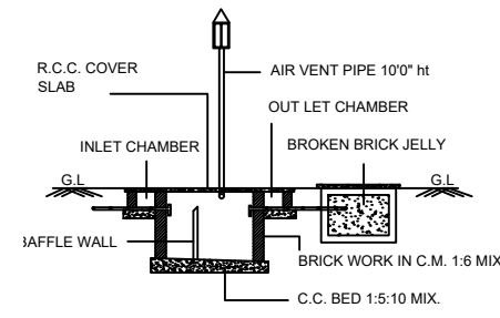
SECTION ON S. TANK & DISPERATION TRENCH
