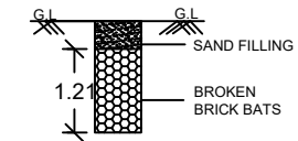
R.W.H.R. PIT DETAILS (NOT TO SCALE)
