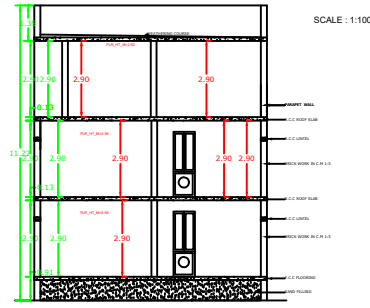
SECTION ON K-S
