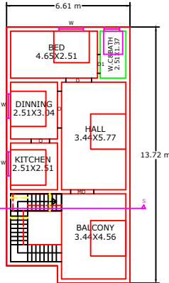
FIRST FLOOR PLAN (Already approved)
