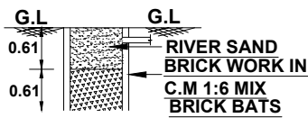
. SECTION ON RAIN WATER COLLECTION TUB .
