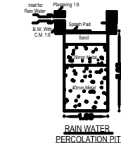
RAIN WATER PERCOLATION PIT
