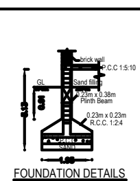
FOUNDATION DETAILS
