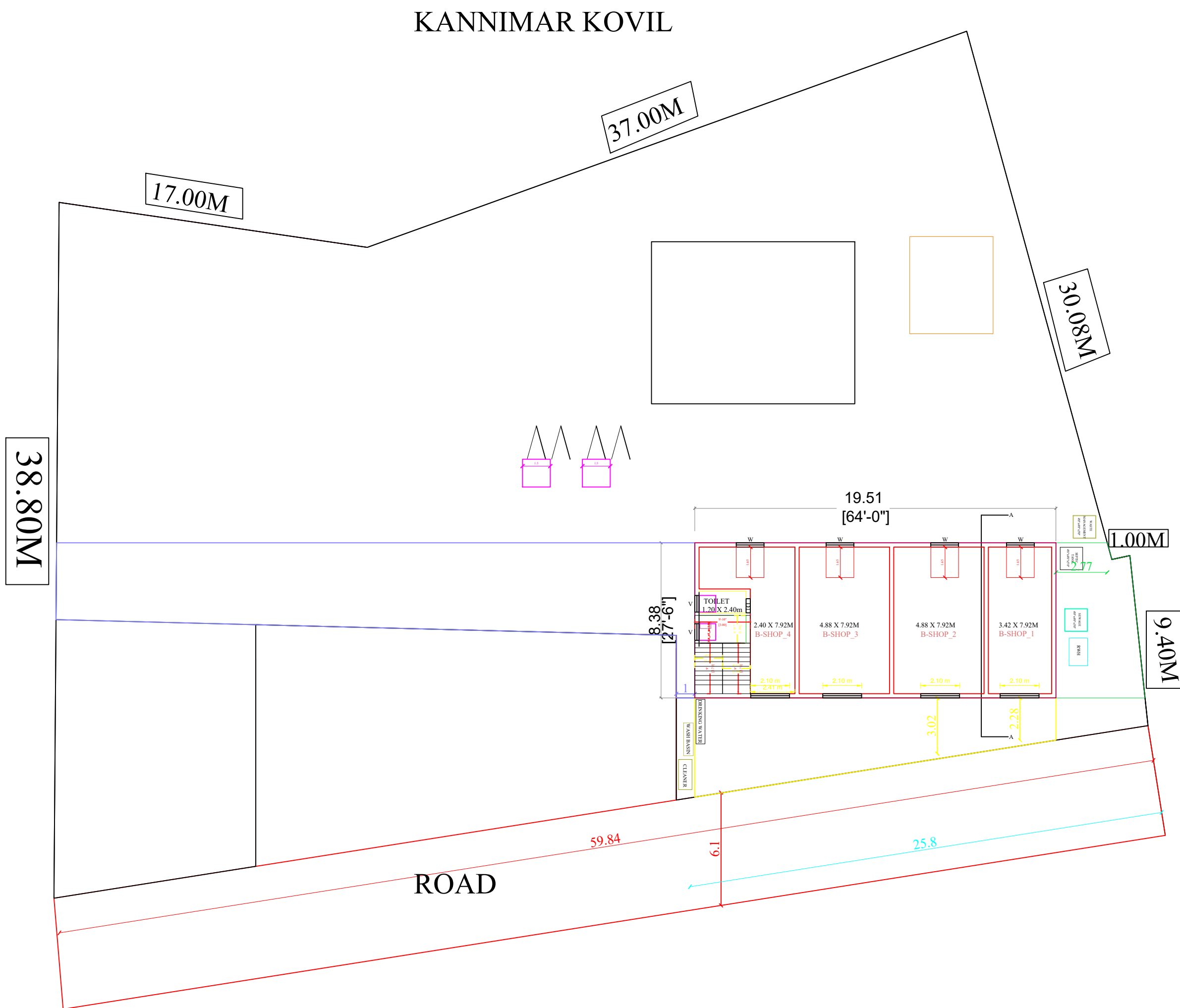
SITE CUM PROPOSED GROUND FLOOR PLAN
