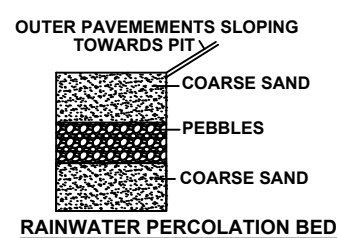
RAINWATER PERCOLATION BED
