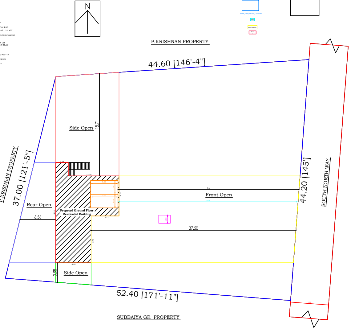
SITE PLAN
