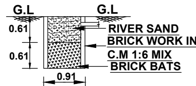
. SECTION ON RAIN WATER COLLECTION TUB .
