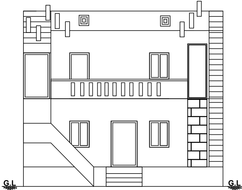
. FRONT ELEVATION .
