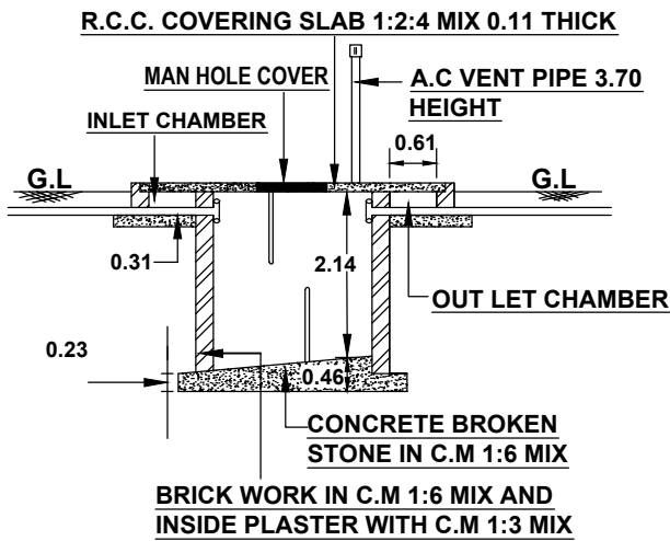
.SECTION ON SEPTIC TANK .
