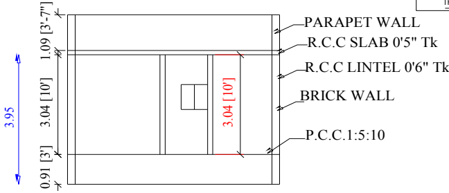
SECTION ON"AB"
