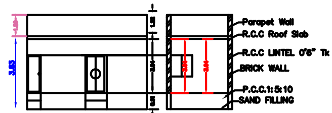
ELEVATION SECTION ON "AB"
