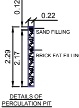
DETAILS OF PERMEATION PIT
