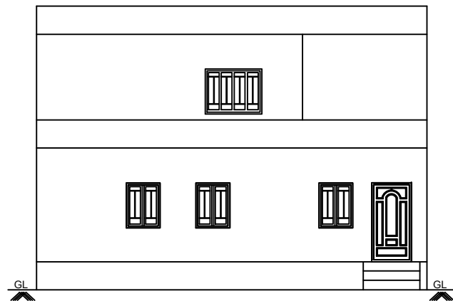
FRONT ELEVATION (EAST FACING)
