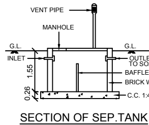
SECTION OF SEP.TANK
