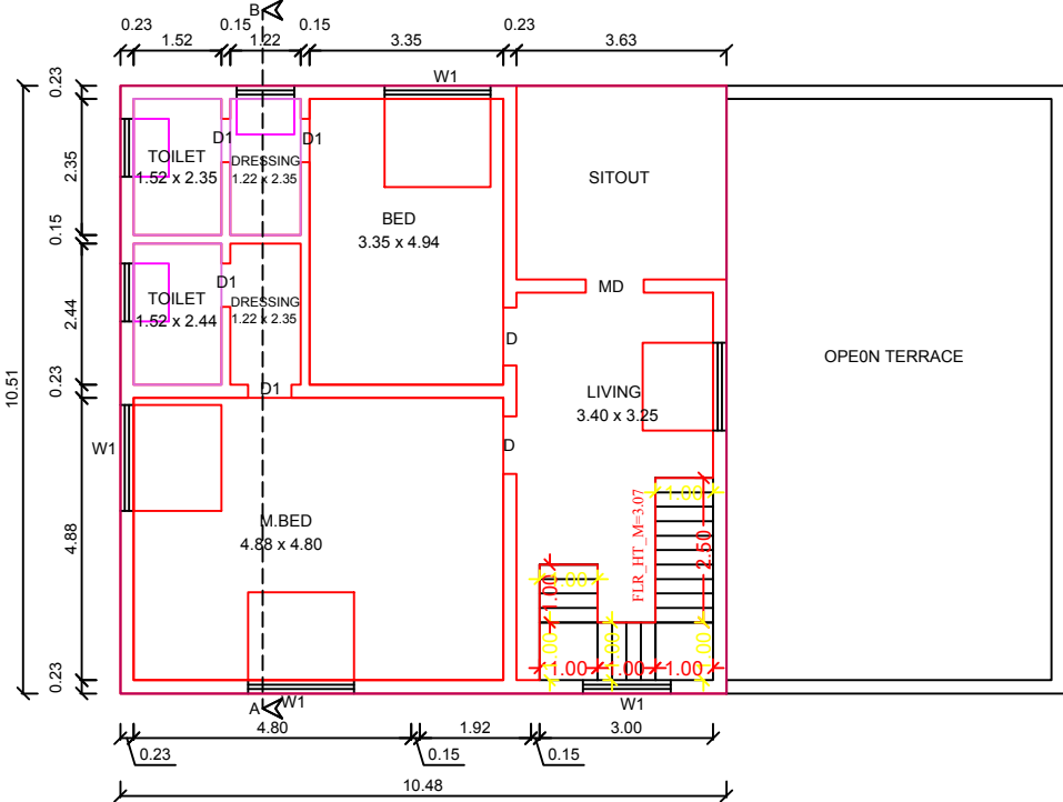
PRO.FIRST FLOOR PLAN
