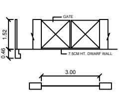
COMPOUND WALL WITH DWAFF WALL DETAILS
