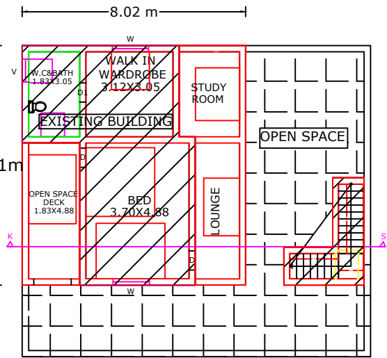
EXISTING SECOND FLOOR PLAN (Already approved) PROPOSED SECOND FLOOR PLAN
