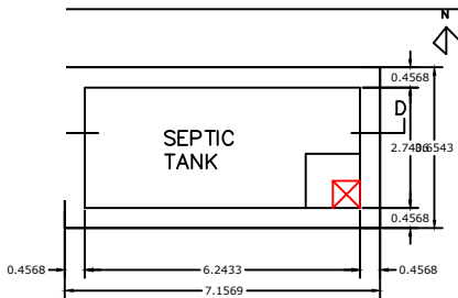
EXISTING GROUND FLOOR PLAN (Already approved)
