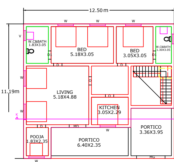
EXISTING GROUND FLOOR PLAN (Already approved)
