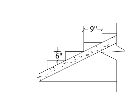
Staircase Detail Not To Scale
