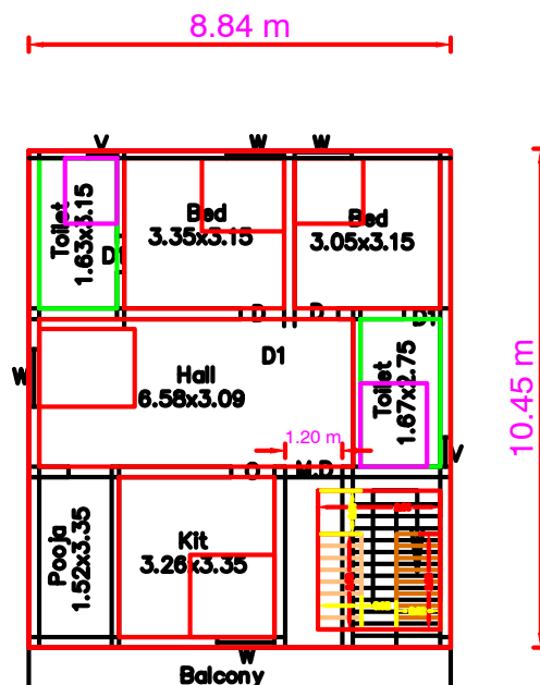
Pro.First Floor
