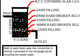
Waste Water Recycle Unit Not To Scale
