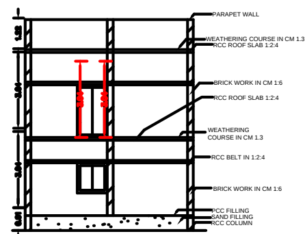
SECTION ON-AA&BB
