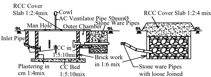
SEPTIC TANK (NTS)
