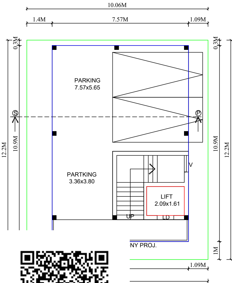
R PLAN
