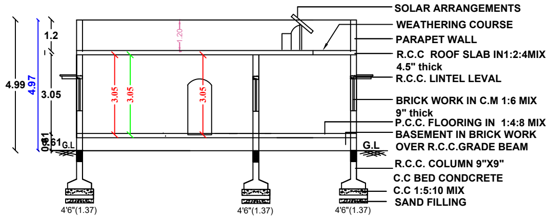
SECTION " AB "
