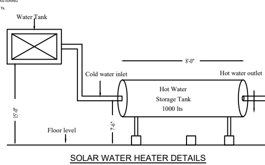
SOLAR WATER HEATER DETAILS
