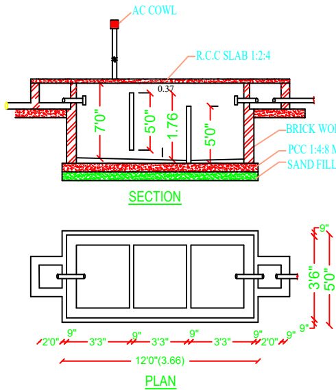
SECTION OF RAIN WATER PERCOLATION BED
