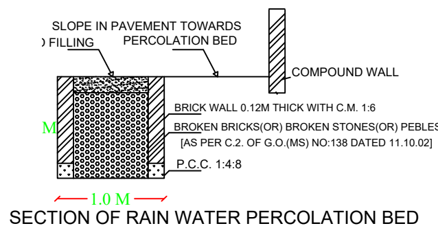
SECTION OF RAIN WATER PERCOLATION BED
