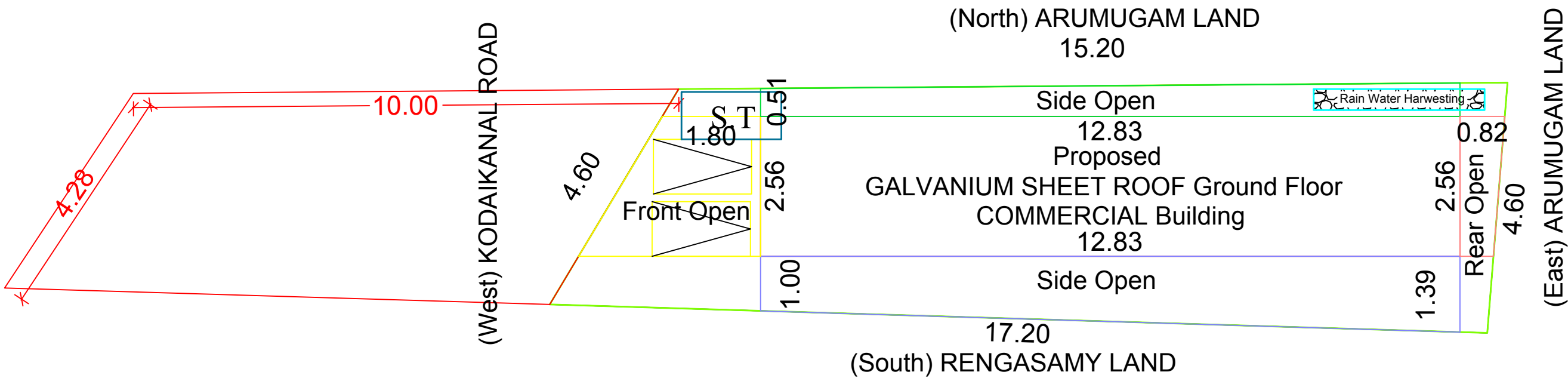
SITE PLAN
