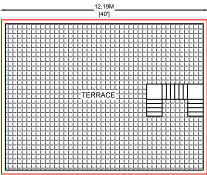
TERRACE PLAN
