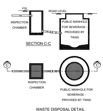
WASTE DISPOSAL DETAIL
