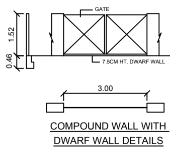
COMPOUND WALL WITH DWARF WALL DETAILS
