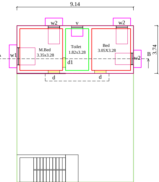
FIRST FLOOR & TERRACE FLOOR PLAN
