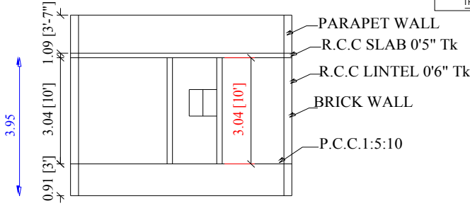
SECTION ON"AB"
