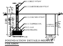
FOUNDATION DETAILS-MID COLUMN
