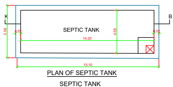
SEPTIC TANK
