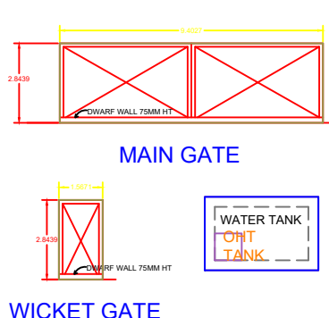
WICKET GATE
