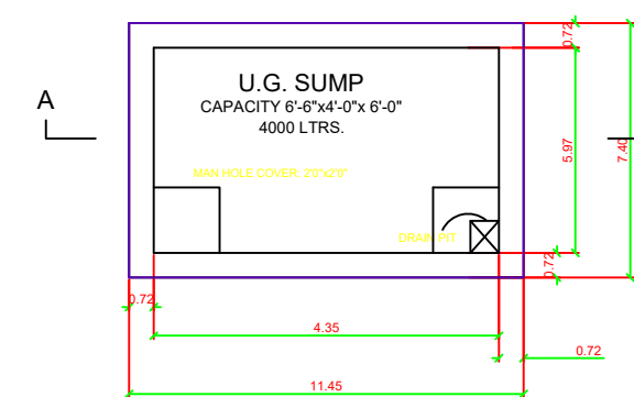
SUMP DETAIL
