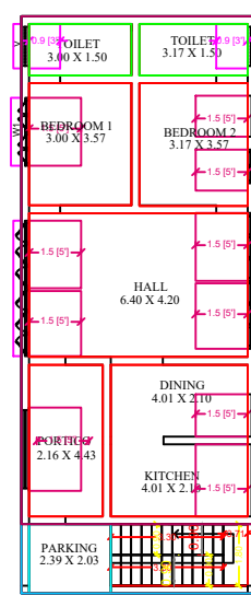
GROUND FLOOR PLAN 1 - Dwelling Unit
