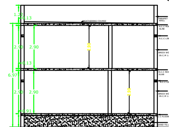
SECTION ON K-S
