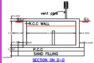
SECTION ON D-D WICKET GATE
