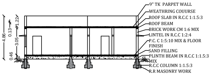
CROSS SECTION ON "A - A"
